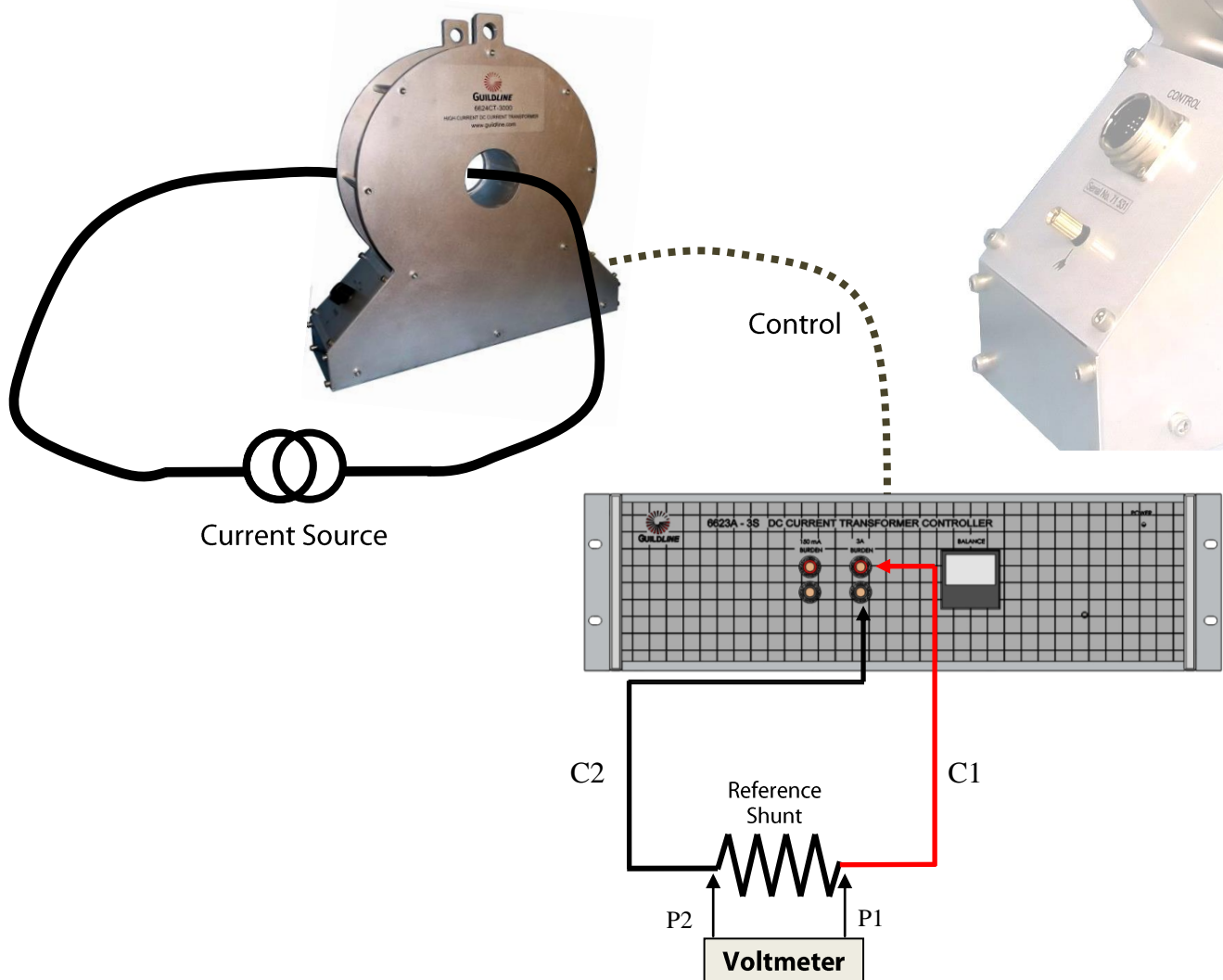
6624CT-3000 Connections
